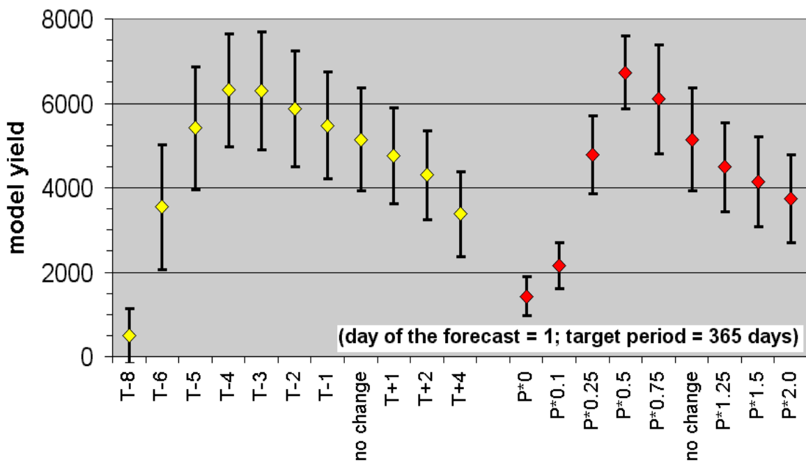
Fig. 8. The same as the previous figure but the synthetic series is generated for the whole year and the changes in temperature and precipitation relate to the whole year, too.
