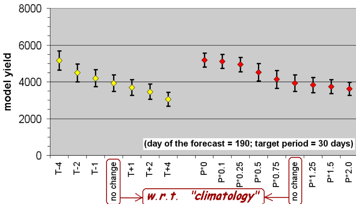
Fig. 5. Sensitivity of the forecast model yields of barley to changes in temperature (T) and precipitation (P). The forecast is given on day D=190 in terms of avg \pm std (vertical bars) and is based on 30 crop model simulations. The input weather series consist of observed weather series till (D - 1) th day of the year and synthetic series since day D . The changes to temperature are additive, the changes to precipitation are multiplicative and the changes to both characteristics are applied to the 30-day period starting on day D . The forecast values are with respect to the mean climatology.
