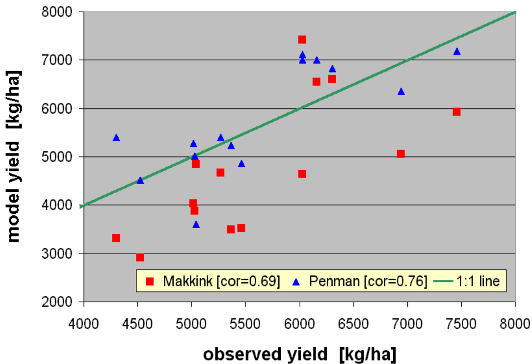
Fig. 2. The same as Fig. 1 but for the winter wheat (Hana), 1985-97.
